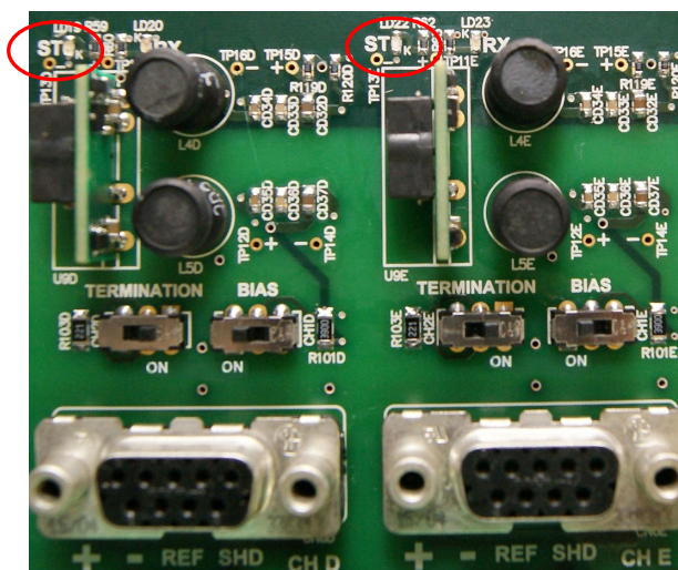
Figure 9 – ST LEDs to indicate the channel status
