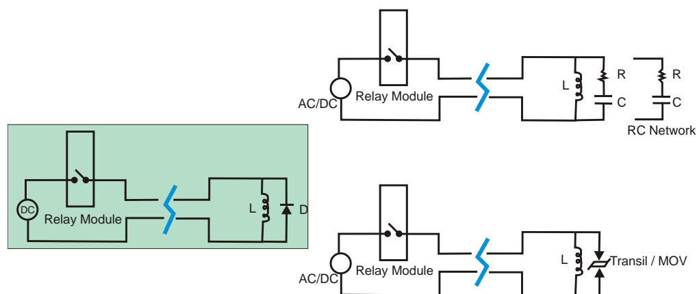
Figure 1.6 – Filters for AC and DC loads
