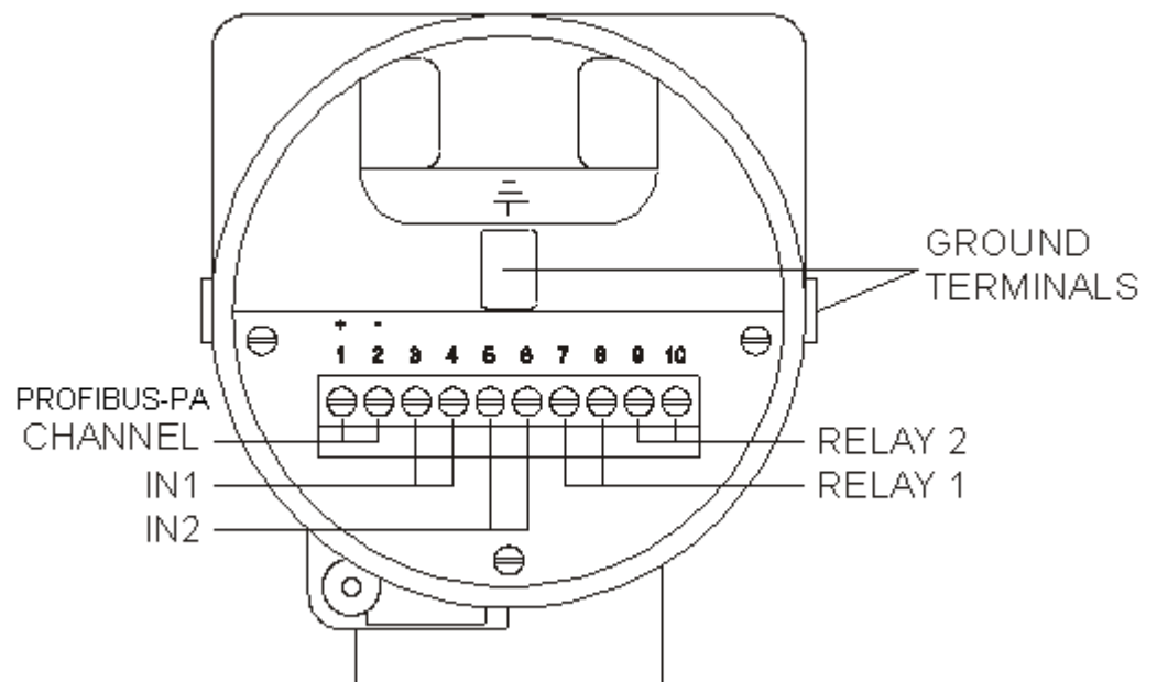
Figure 1.3 – Terminal Block
