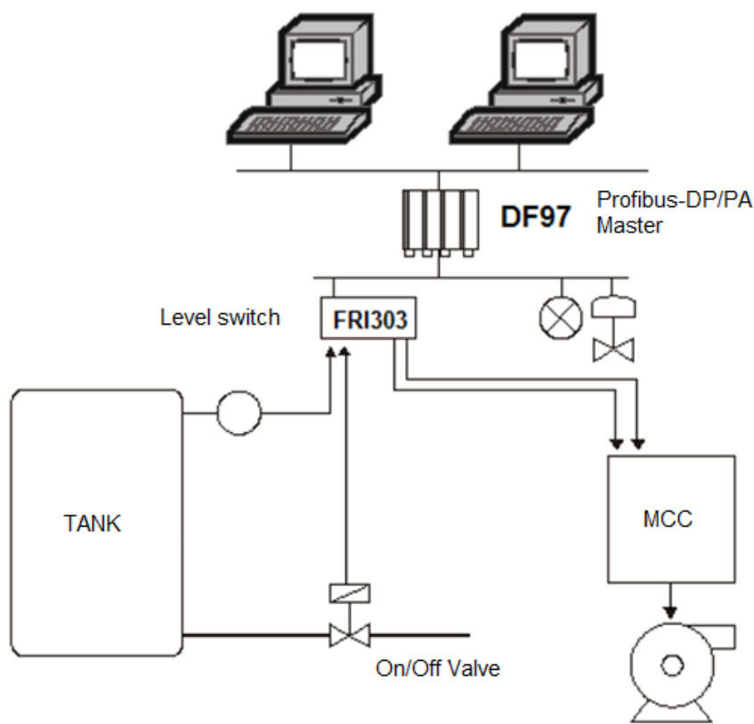
Figure 3.5 – FRI303 – Application 3
