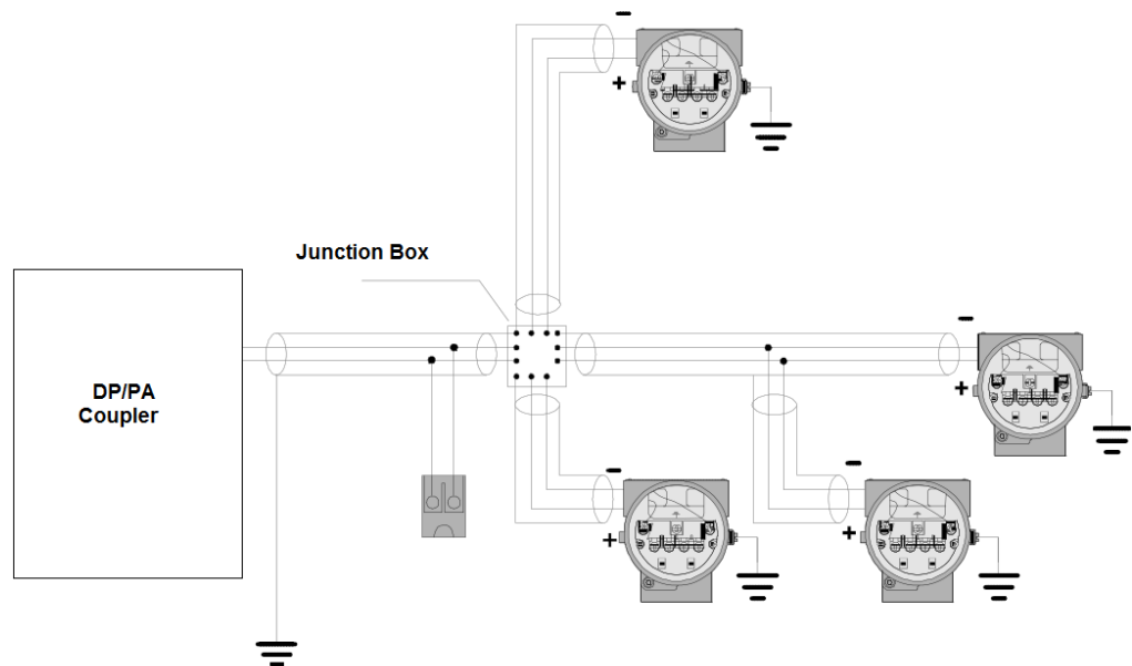
Figure 1.11 - Bus Topology
