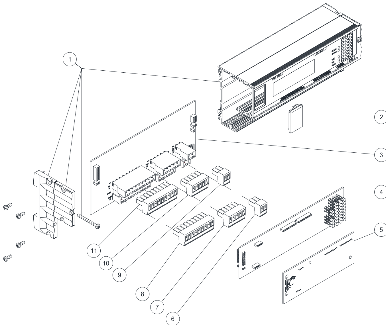
Figure 4.1 – Vista Explodida do DC303
