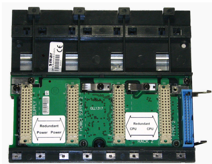
Figura 3. 24 - Rack – DF78
