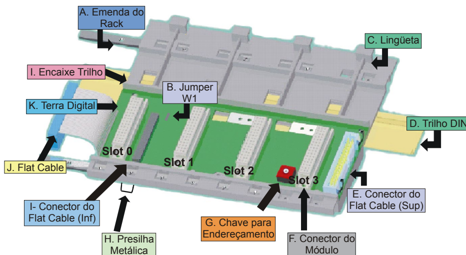
Figura 4. 1 – Rack DF1A
