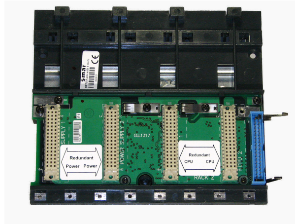
Figura 14. 6 – Rack DF78
