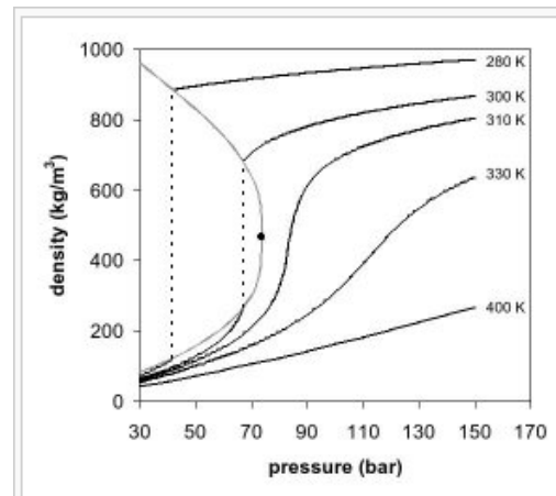
Figure 2. Carbon dioxide density-pressure phase diagram
