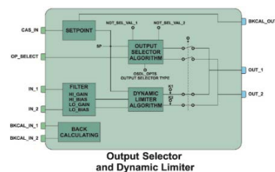
Output Selector and Dynamic Limiter
