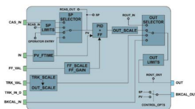
Advanced PID
